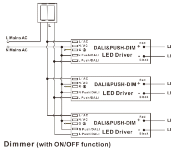
DALI Dimming Wiring Diagram1
