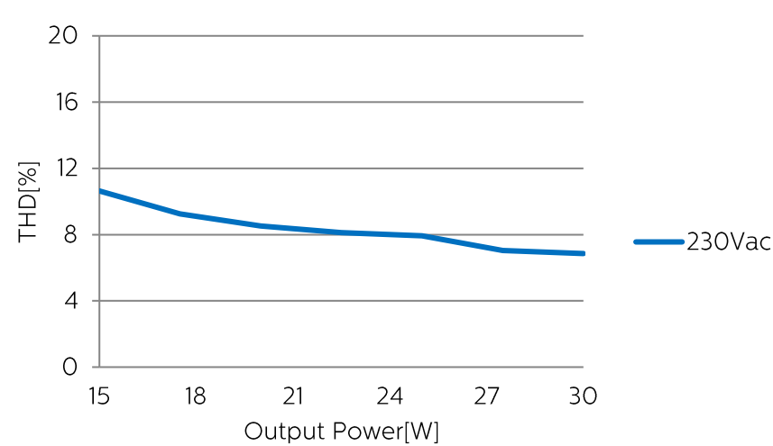
THD versus output power
